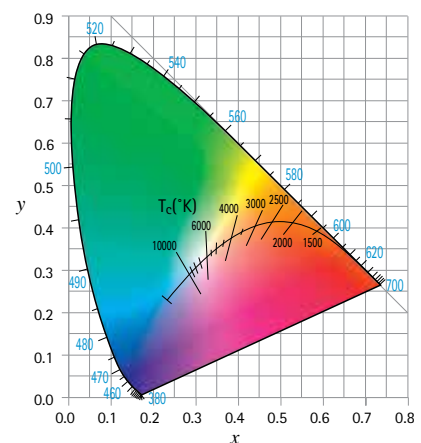
Diagram 1: Planckian Locus
